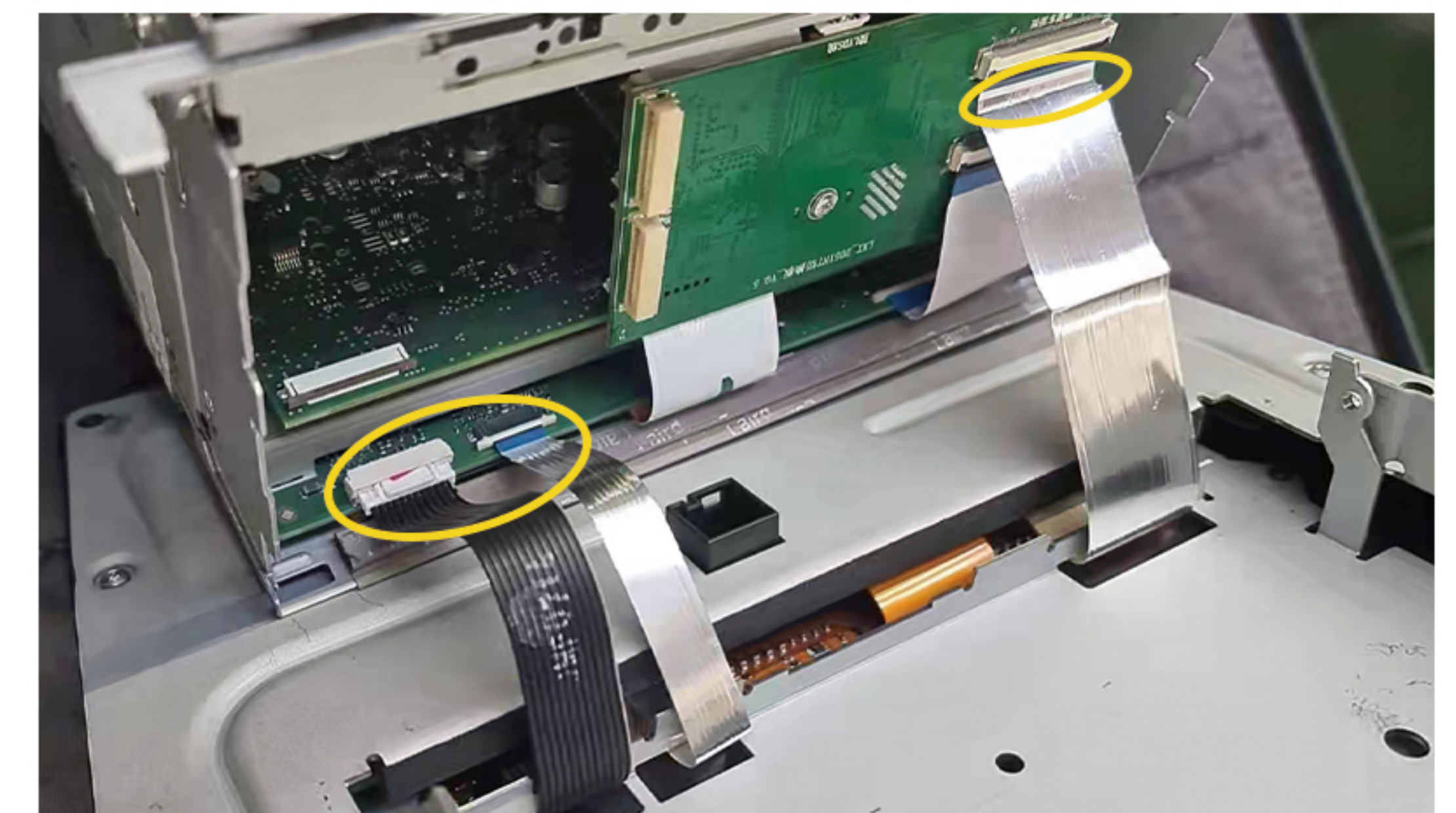
3: Finally restore three factory wires. 50P FFC and 12P wiring into new PCB and SD card wire. Restore panel and screws.
