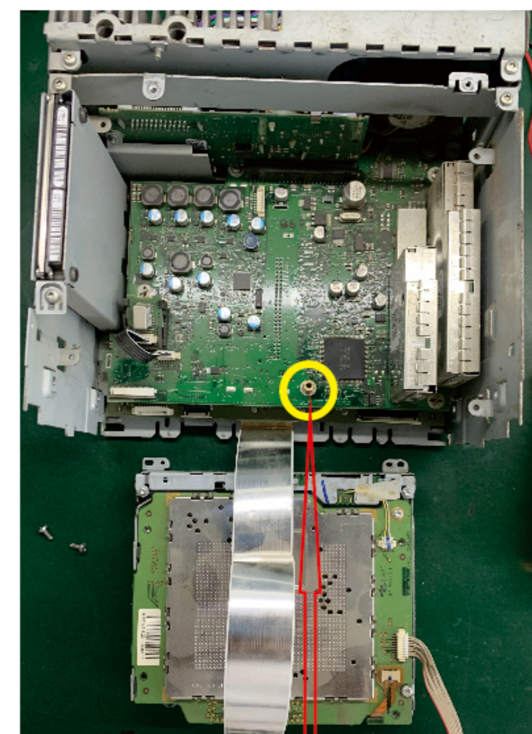
1: Separate car panel and headunit, then unscrew core screws then unscrew the highlighted screw to add PCB
