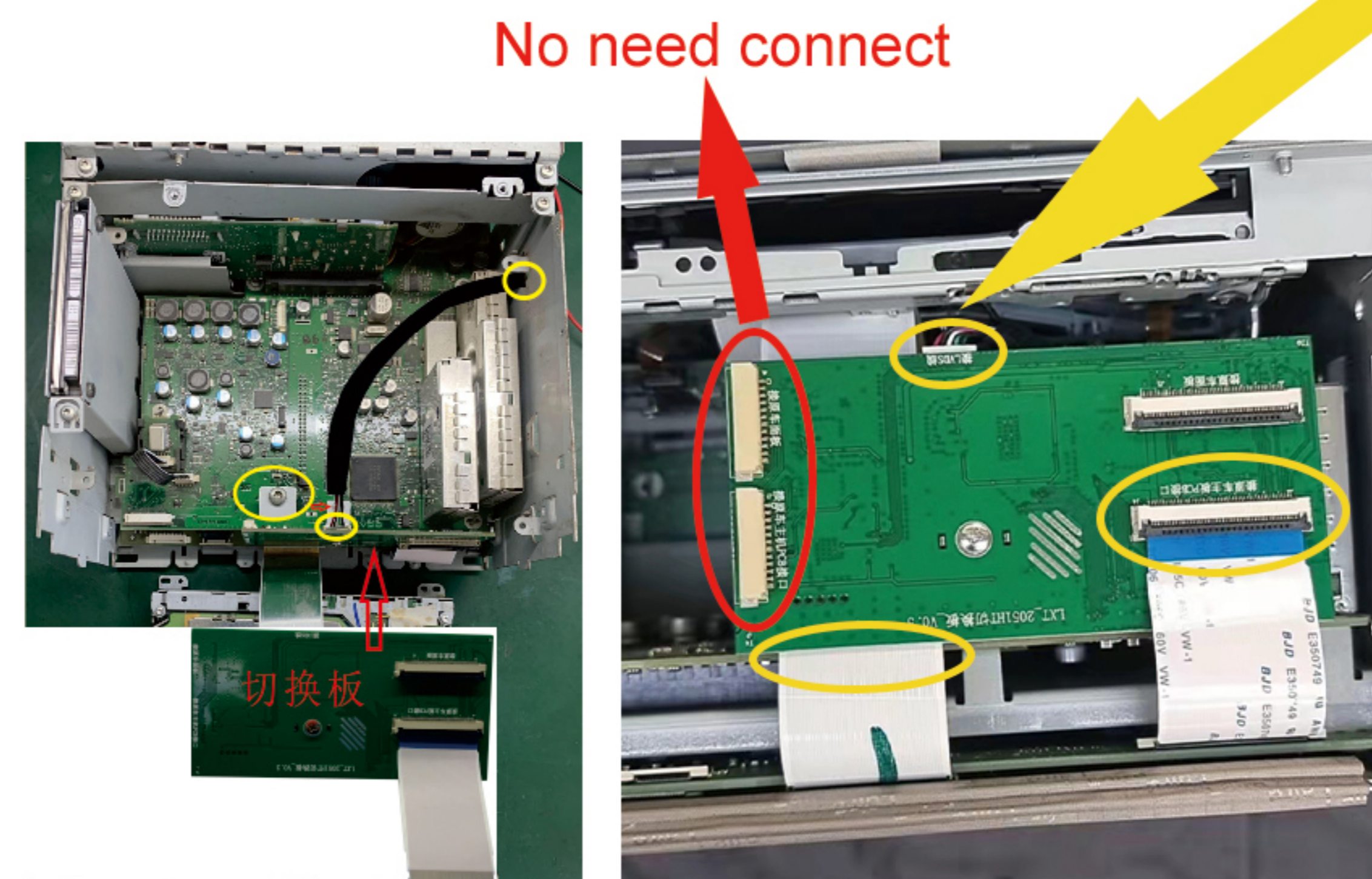
2: Take out PCB from package and install it in the slot, secure with a screw. Insert 50P FFC into factory slots. Plug LVDS wire and pay attention to headunit entry location. Make sure all wiring are flat to avoid circuit shorting. Restore panel. Result is the picture on the right.
